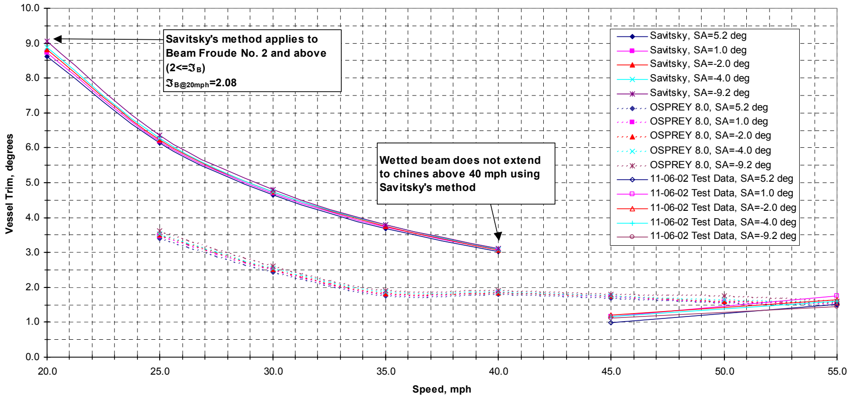
Vessel Trim vs Speed for a range of shaft angles (SA) comparing Savitsky's Method, OSPREY 8.0 planing code, and 11-06-02 test data
